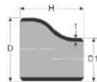
red_con_ec c_dim
