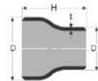
Reducer concentric
