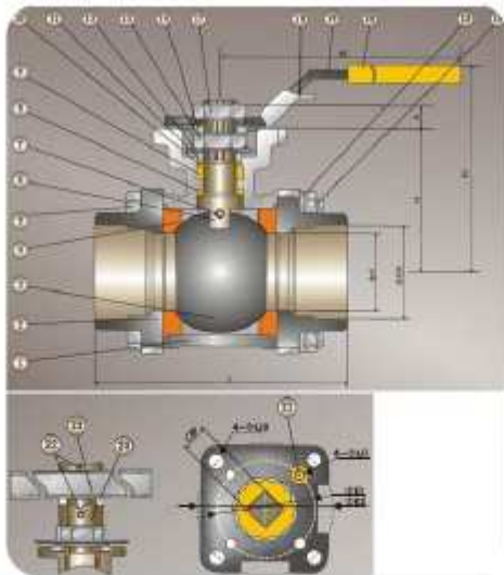
2PC-Socket-Weld-Ball-Valve2
