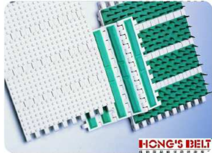
Modular_plastic_conveyor_belt_small
